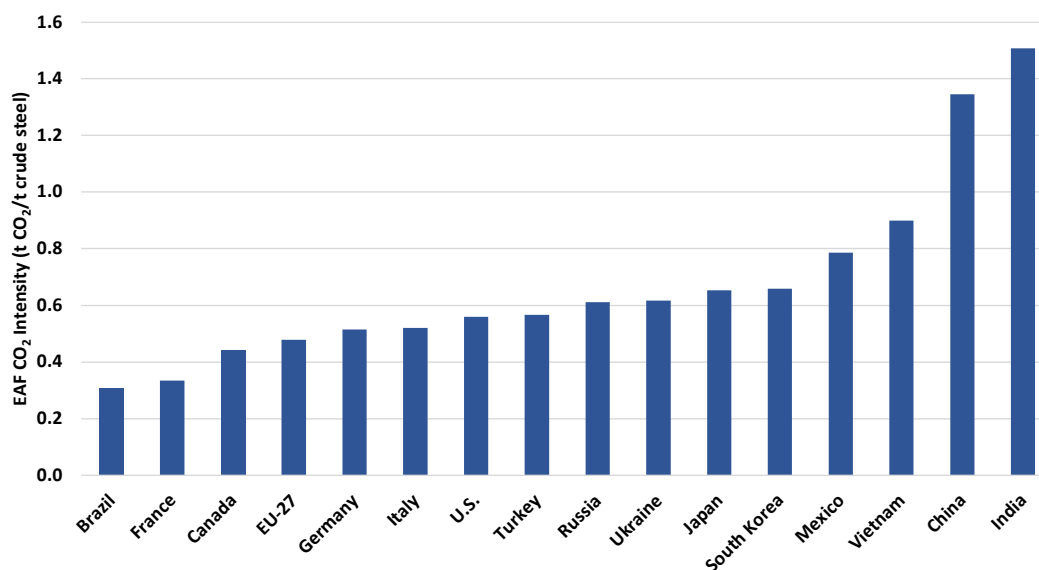
Figure 11. The CO 2 intensity of EAF steel production in the studied countries/region in 2019
