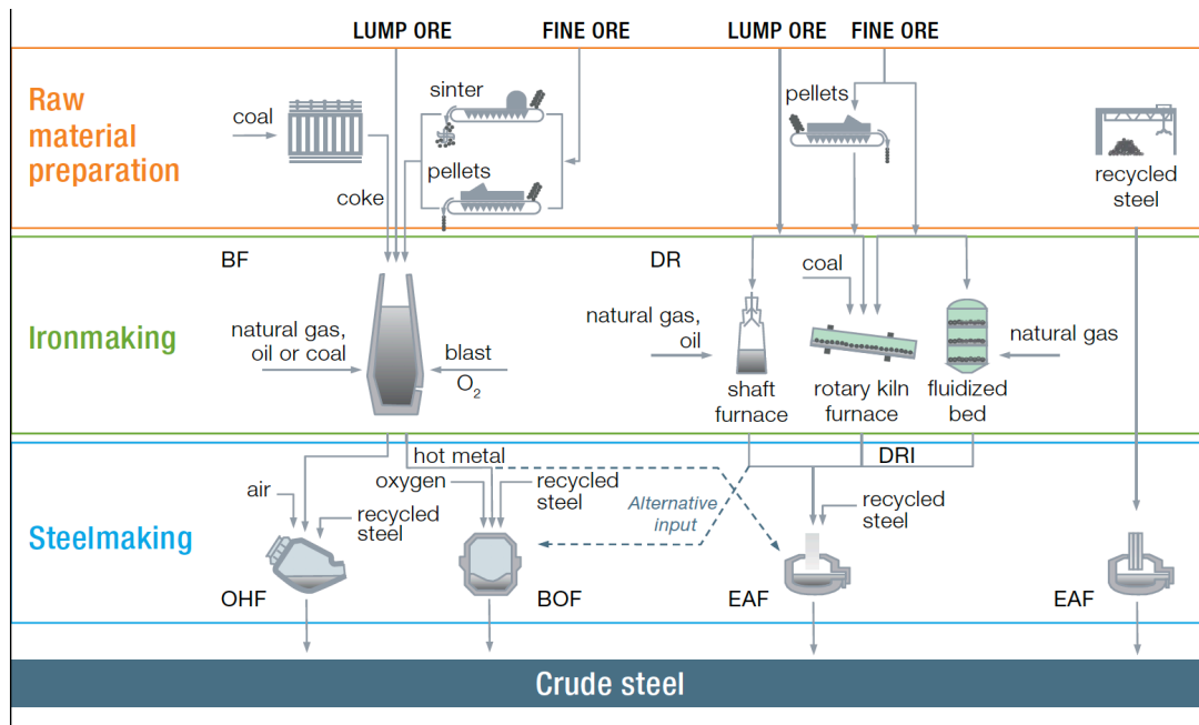
Figure 1. Steelmaking production routes (Worldsteel 2019)
