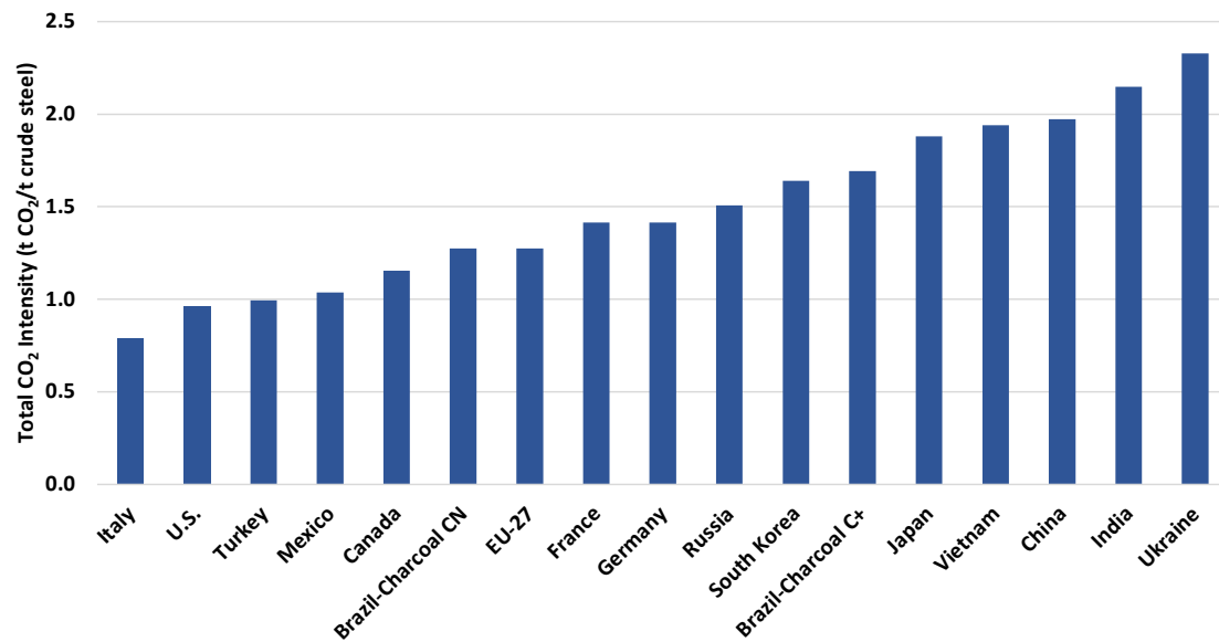
Figure 7. Total CO 2 emissions intensity of the steel industry in the studied countries/region in 2019 Note: Brazil-Charcoal CN refers to when charcoal is considered carbon neutral. Brazil-Charcoal C+ refers to when charcoal is not considered carbon neutral because of questions and concerns regarding the sustainability of biomass used in the steel industry in Brazil. See methodology in Appendix for more information.
