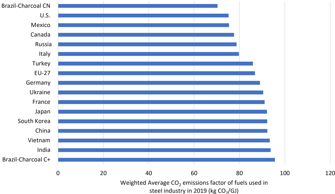
Figure 9. Weighted average CO 2 emissions factors of fuels in the steel industry in the studied countries/region in 2019
