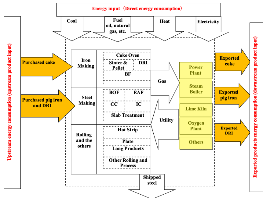
Figure A.1. Flow chart of iron and steel sector boundaries used in this study
