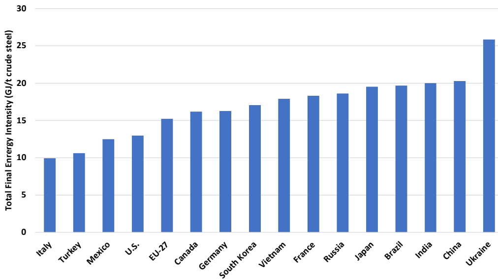
Figure 5. Total final energy intensity of the steel industry in the studied countries/region in 2019
