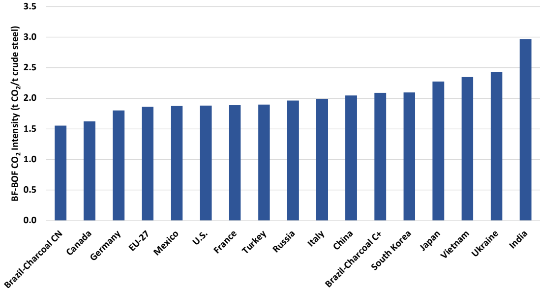
Figure 8. The CO 2 intensity of BF-BOF steel production in the studied countries/region in 2019 Note: Brazil-Charcoal CN refers to when charcoal is considered carbon neutral. Brazil-Charcoal C+ refers to when charcoal is not considered carbon neutral because of questions and concerns regarding the sustainability of biomass used in steel industry in Brazil. See methodology in Appendix for more information.
