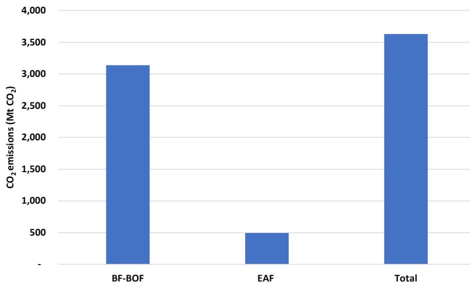
Figure 4. Global steel industry CO 2 emissions in 2019 by process type (source: this study)
