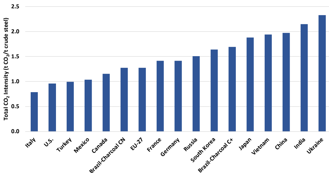
Figure ES1. The CO 2 intensity of the steel production in the studied countries/region in 2019
