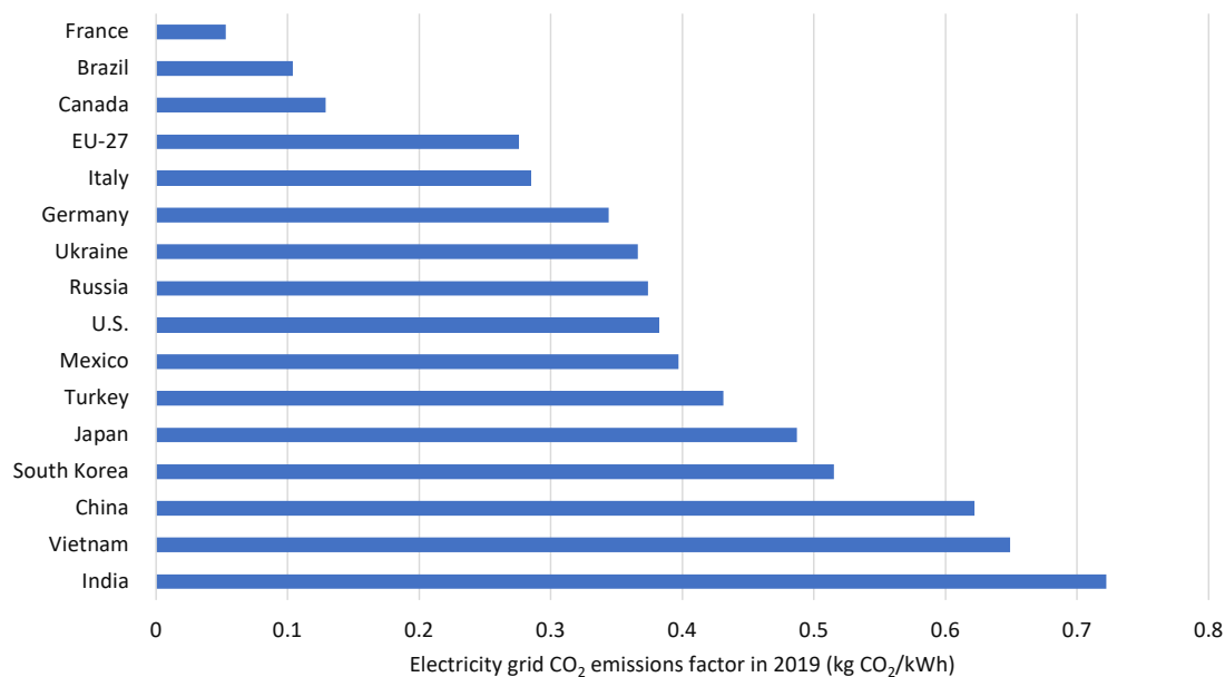
Figure 10. Electricity grid CO 2 emissions factors in the studied countries in 2019 (IEA 2021)
